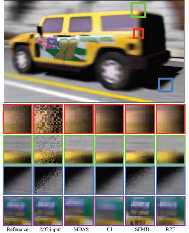
Fig. 12. This motion-blurred CAR scene was rendered at 4 spp with various algorithms (top image is from RPF). The first row of insets shows a region where compressive integration (CI), sheared-filter motion blur (SFMB), and RPF all work well. In the second row, SFMB reconstructs detail in the back wall that our algorithm overblurs, but it also leaves noise on the roof of the car that RPF removes. The third inset is left noisy by SFMB but is denoised by ours. Finally, the fourth row shows a static region of the scene that should be sharp but is overblurred by the CI approach. The full images are available in the technical report [Sen and Darabi 2011b].
