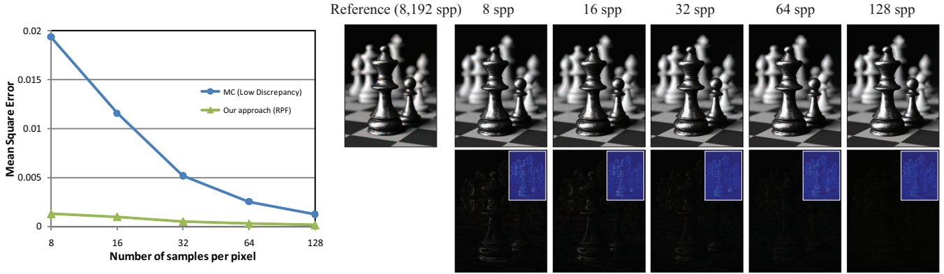
Fig. 14. Convergence of RPF to the ground truth as we increase the number of samples. On the left we show a plot of MSE versus the number of samples for standard MC and for our approach. Unlike Fig. 15, MDAS was excluded because it took too long for this scene at higher sampling rates. On the right we show the output of our algorithm in the top row, and difference images (with “heat” image insets) that compare our results to the reference in the bottom.
