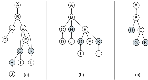
Figure 3: A DAG is shown in (a) with multiply-referenced nodes drawn shaded. The dominator tree for this DAG is shown in (b). Node B is the parent and therefore the immediate dominator of H . Similarly, E is the immediate dominator of both G and K . The partial dominator tree in (c) is obtained from the tree in (b) by keeping only the multiply-referenced nodes, their immediate dominators, and the root.
