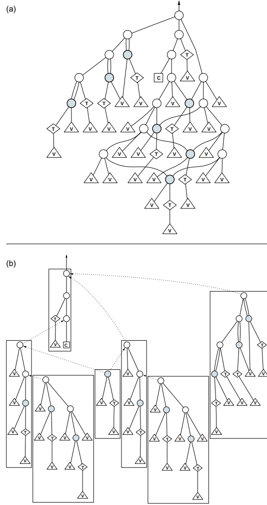
Figure 5: (a) DAG of the RBP shader, after instruction selection. (b) A partition of the shader with 7 passes, computed by RDS for the ATI Radeon 8500 architecture. Texture fetches (T), vertex interpolants (V), and constants (C) are shown as diamonds, triangles and squares, respectively. Circles represent other fragment operations, and multiply-referenced nodes are shaded. Dotted edges indicate dependencies between passes.
